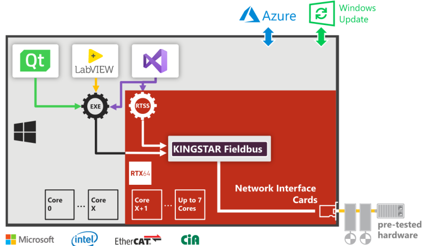
KINGSTAR Fieldbus powered by EtherCAT Architecture
